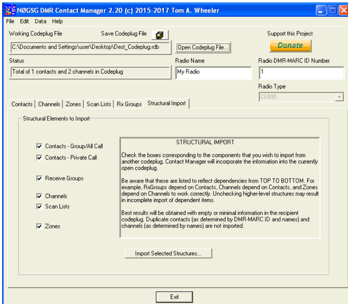
Figure 10: Structural Import Tab
