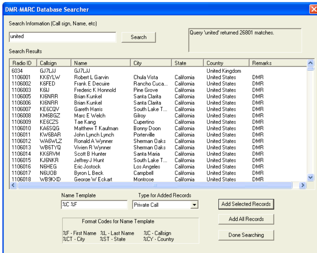
Figure 4: Database Search Dialog
