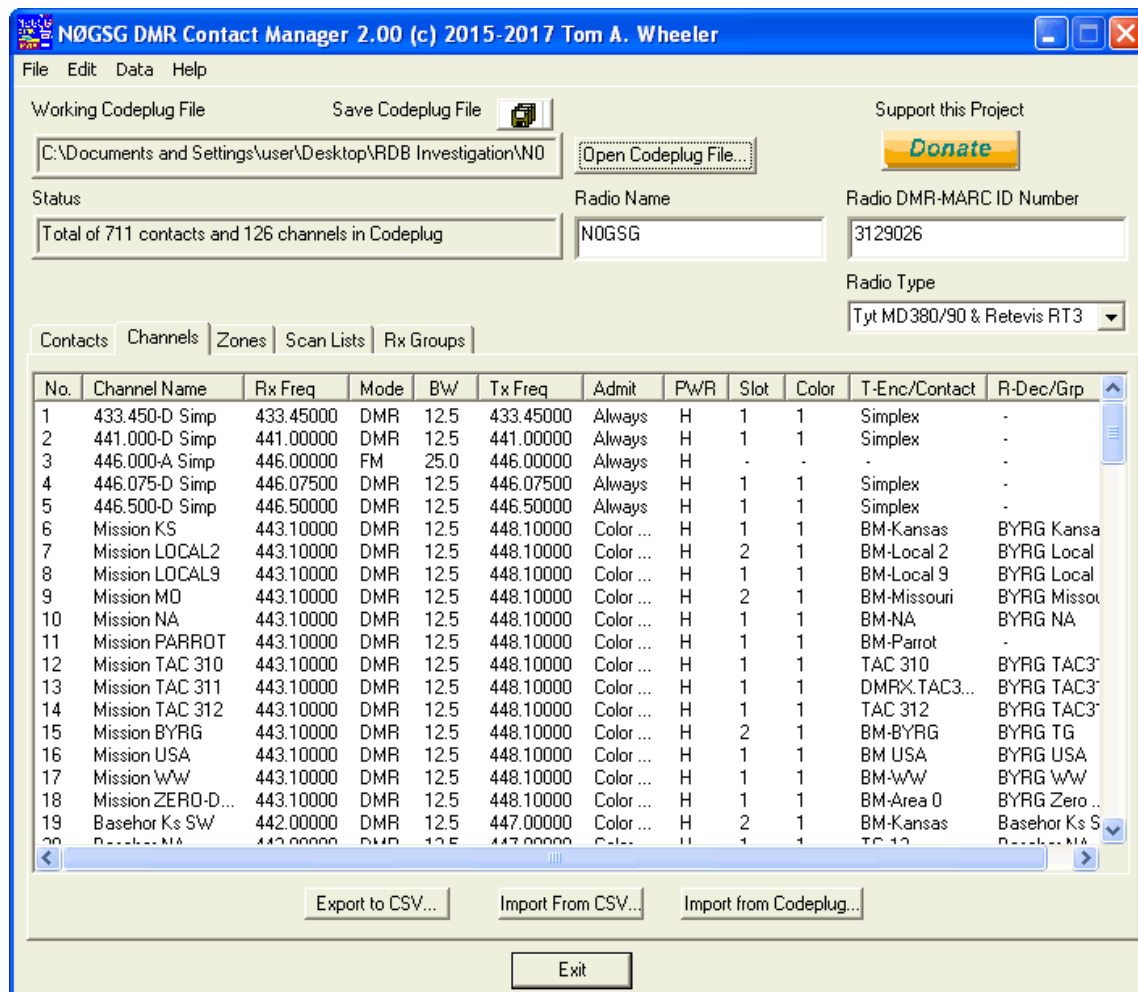
Figure 5: Contact Manager in CHANNEL Mode
