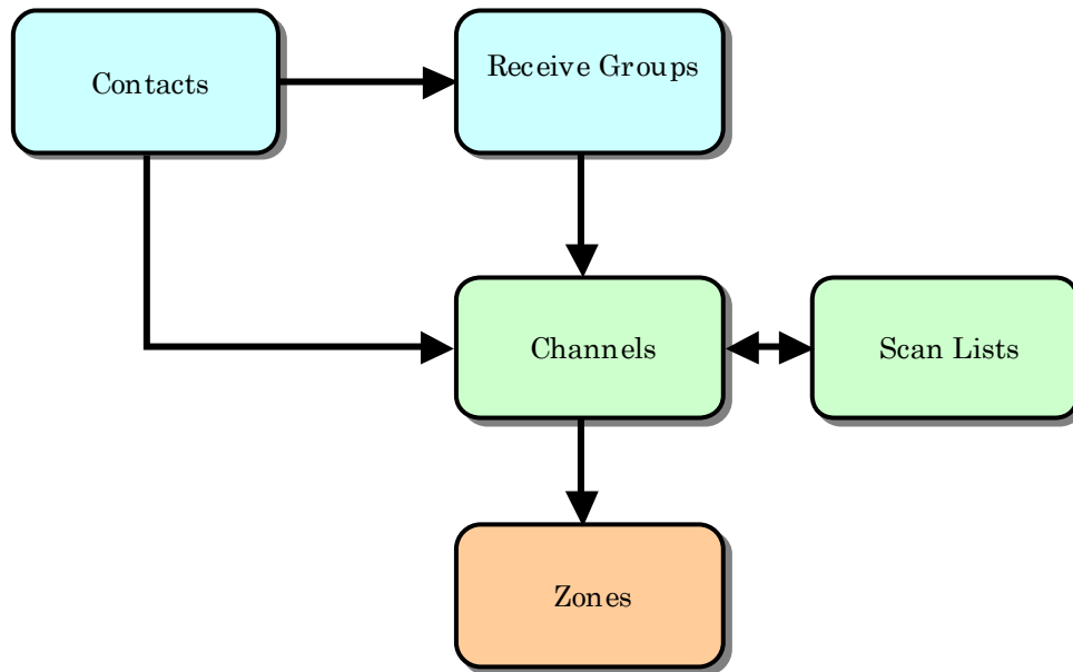
Figure 9: Codeplug Data Dependencies
